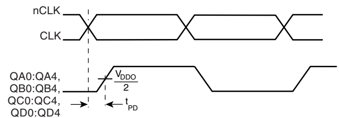
PROPAGATION DELAY
